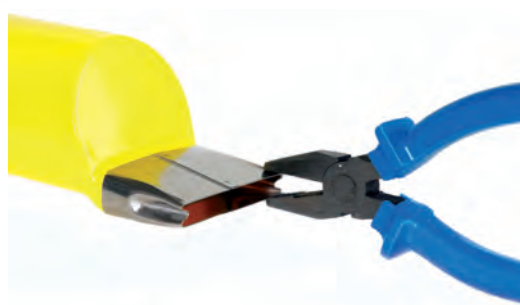
2. Adjust the nozzle width with pliers
