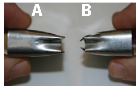
3. Sides of nozzle can be notched for: A - a raised or overfilled joint B - narrow floor tile joints
